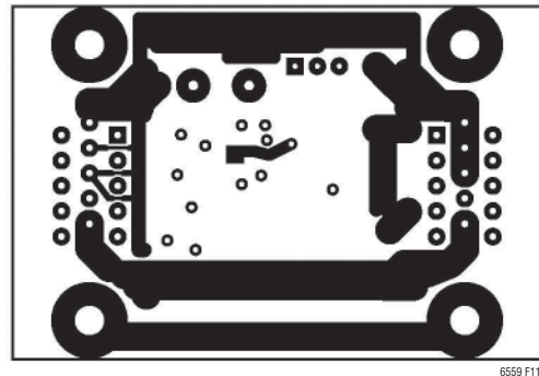
Figure 11. DC1063A Bottom Side
